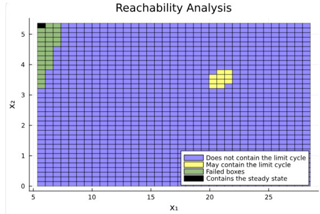
Fig. 1: Projection of the cross-section, that maps onto itself, showing the geometric classification results. The black box contains the steady-state point and was excluded from the reachability analysis. The blue boxes is the region that does not contain the limit cycle. The cluster of yellow boxes signify the region that may contain the limit cycle. The green boxes are classified as the boxes that failed to return a solution for reachability analysis due to solver crash or blow up in the bounds due to overapproximation. The system parameters used in the simulation are: \alpha = 26.26 , \gamma = 0.92 , k = 4 , n = 5 .
