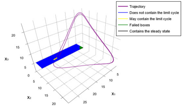
Fig. 2: The numerical solution of the three-gene cyclic regulatory network with initial condition (19, 3.5, 5.361) passes through the region classified as "May contain the limit cycle" in Fig. 1. The system parameters used in the simulation are: \alpha = 26.26 , \gamma = 0.92 , k = 4 , n = 5 . x, y, z axes represent the concentration of i -th (for i = 1, 2, 3 ) protein respectively.
