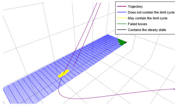
Fig. 3: A magnified view of Fig. 2 showing the intersection of the numerical solution with the boxes classified as “May contain the limit cycle”.
